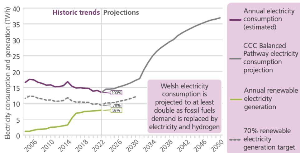
Figure 28 Comparison of annual Welsh electricity consumption and generation trends against the 70% target. Source: Welsh Government, 2023a.
