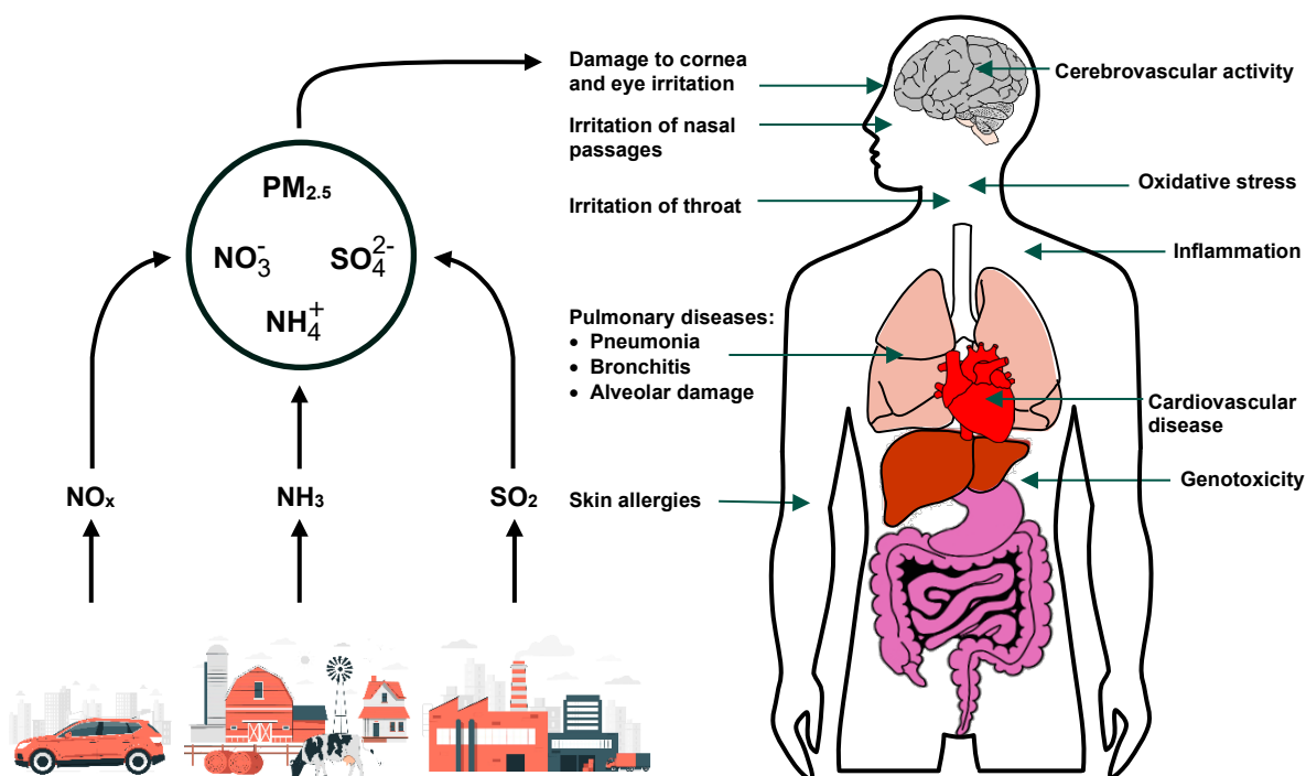
Figure 37: \text{NH}_3 reacts with other gases in the atmosphere, primarily nitrogen oxides ( \text{NO}_x ) and sulphur dioxide ( \text{SO}_2 ), to form secondary particulate matter ( \text{PM}_{2.5} ).
